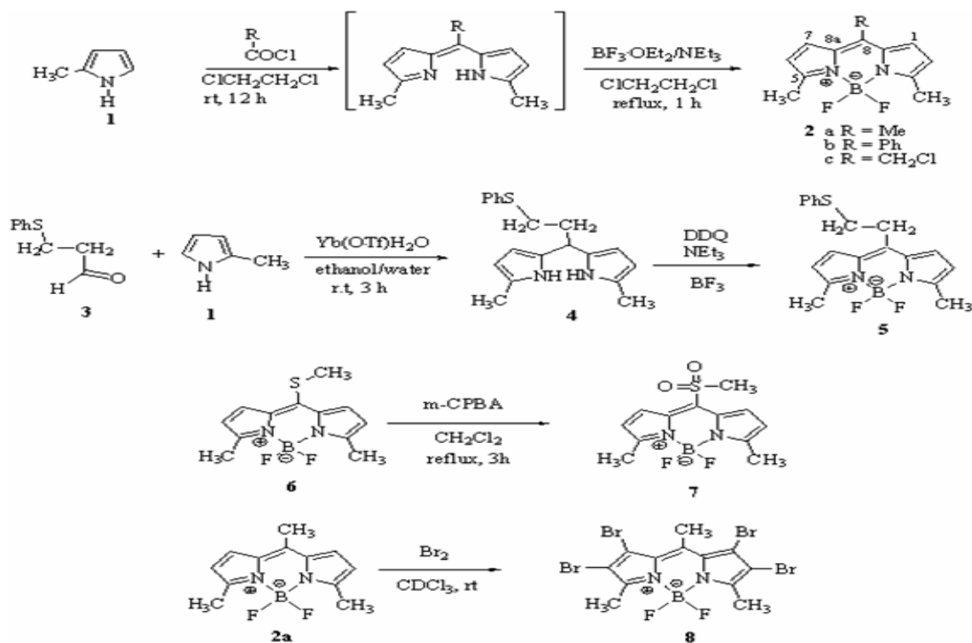
Scheme: Synthesis of 8-substituted 4,4-difluoro-4-bora-3a,4a-diaza-s-indacene dyes.
